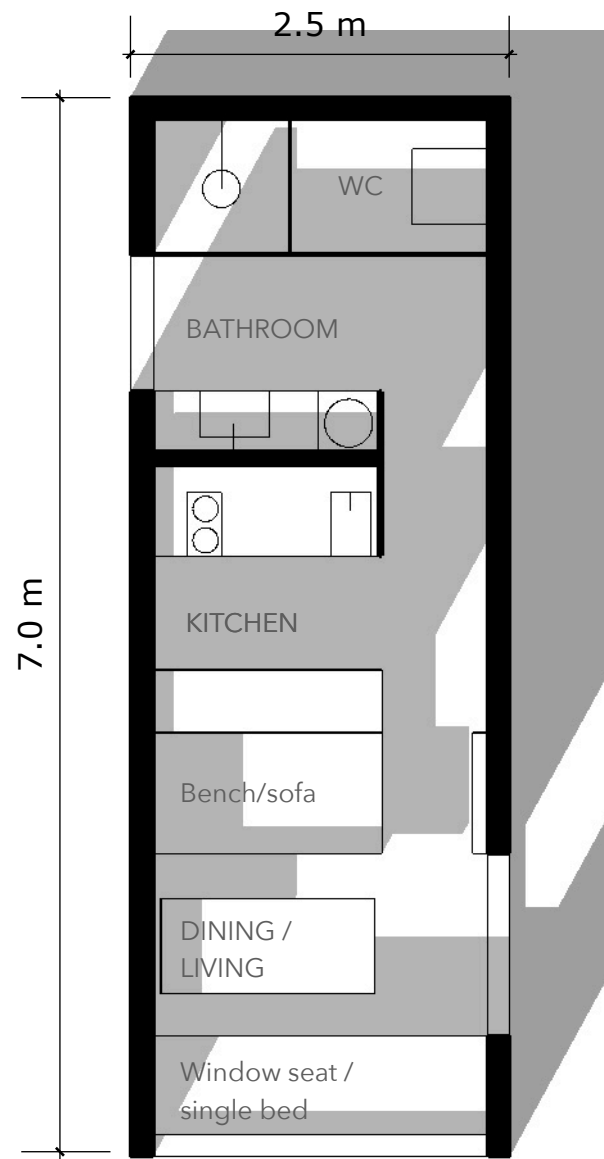
GROUND FLOOR PLAN Scale 1:50
